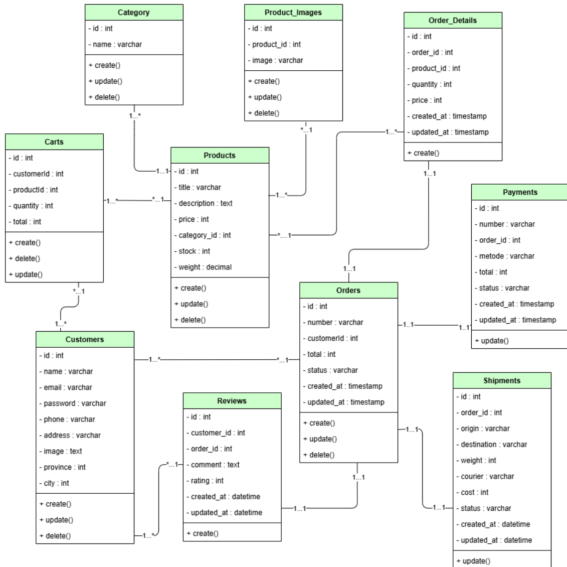
Figure 7. Class Diagram
